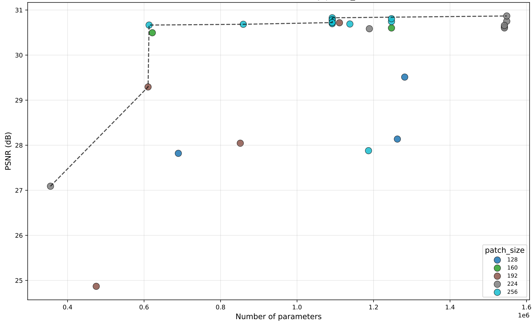
PSNR vs #Params — HAT — by patch_size
